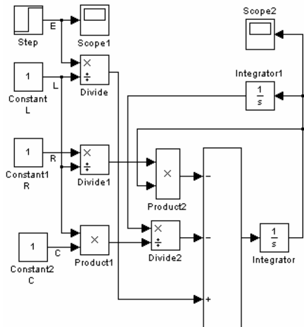
Fig. 13 A model for the classic electrical circuit RLC (Fig. 9) described in Simulink®
