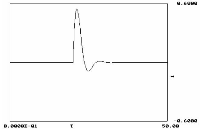
Fig. 12 The output of the PLOTXY(t, i) statement
