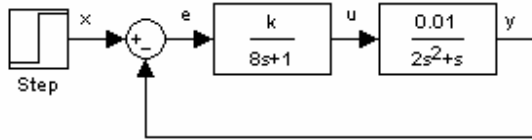
Fig. 15 A control loop block diagram
