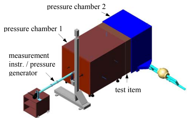
Fig. 3 Experimental setup “MSRCMT”
