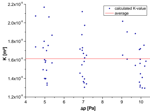
Fig. 16 Permeability of rock wool at forced flow-through
