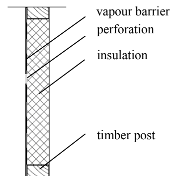
Fig. 4 Schematic layout of the double layer wall specimen
