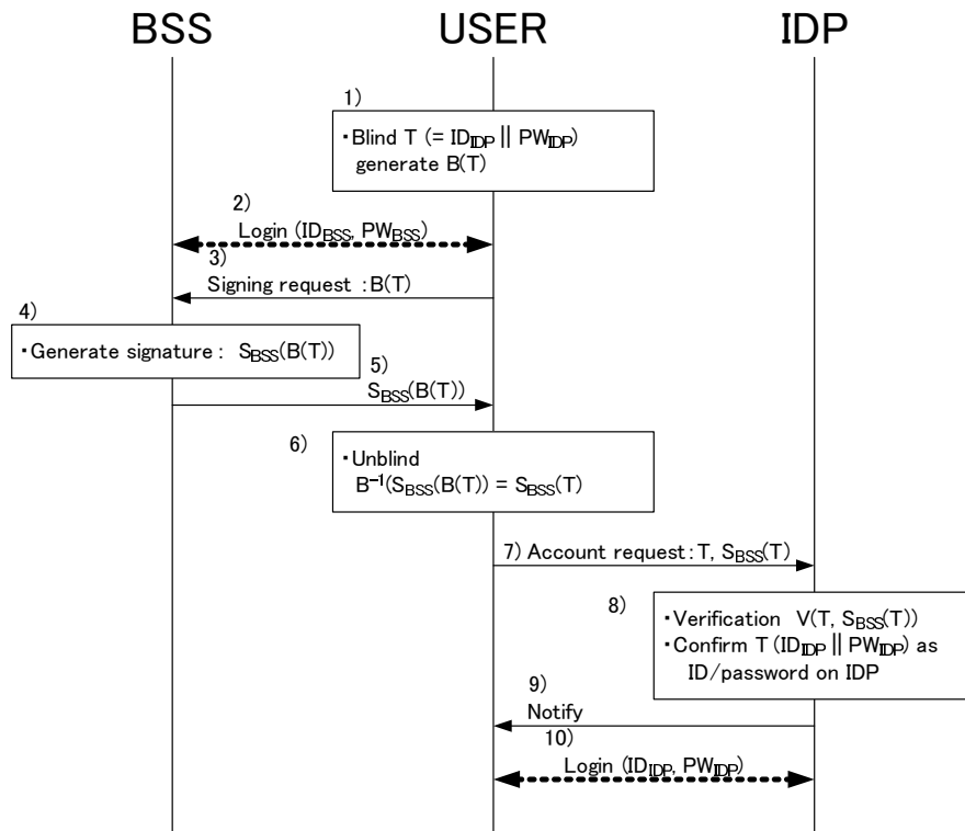
Fig. 3. Sequence of PseudoID account management
