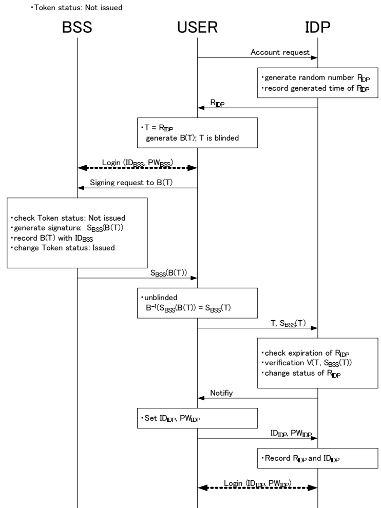
Fig. 5. Account generation sequence of the proposed method
