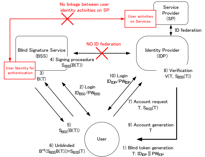
Fig. 2. Schematic representation of PseudoID account management
