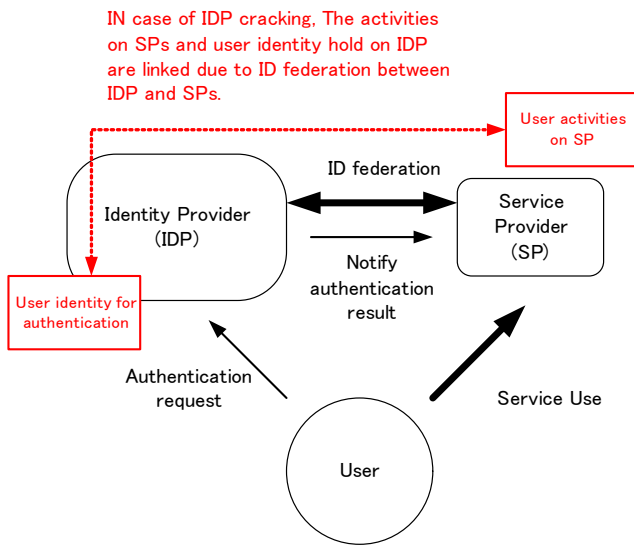
Fig. 1. Privacy problem on SSO by ID federation
