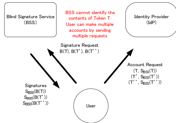
Fig. 4. Problem of multiple account generation on PseudoID
