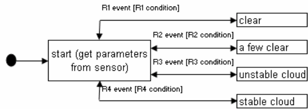
Fig. 8 Fuzzy state diagram for weather condition
