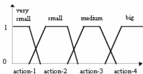
Fig. 5(a) Fuzzy action and concrete action
