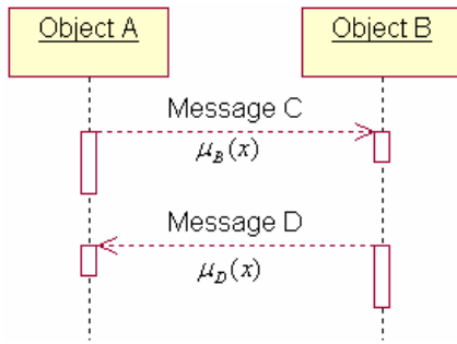
Fig. 4 The fuzzy messages in F-UML
