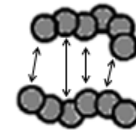
Fig. 2 Attractive interactions between the connected segments in PC-SAFT EOS
