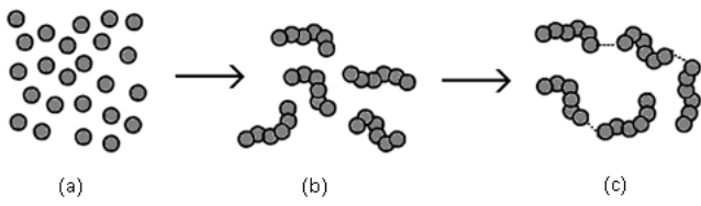
Fig. 1 Schematic representation of SAFT theory: (a): equal-sized spherical segments; (b): formed molecule chains; (c): hydrogen bonding between chains.
