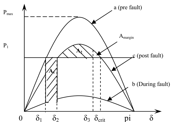
Fig. 8 power Vs angle curve without compensation
