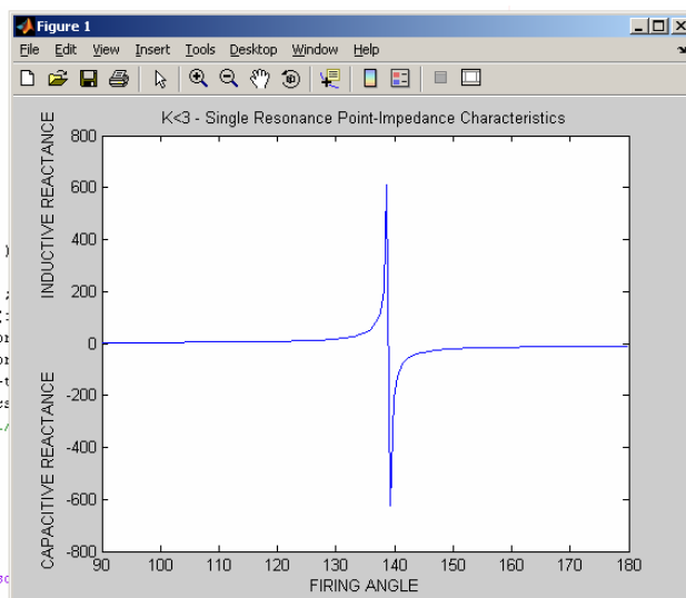
Fig. 4b C = 247.5 \mu F, L = 8.5mH
