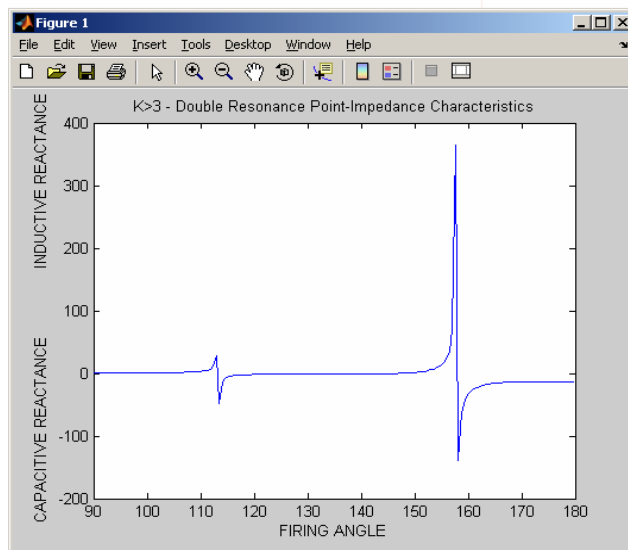
Fig. 4c C = 247.5 \mu F, L = 2.5mH
