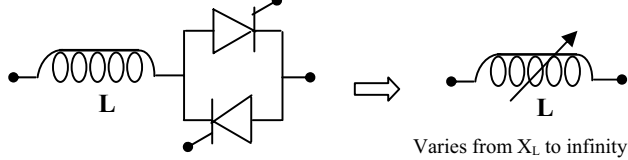
Fig:2 Equivalent circuit of TCR
