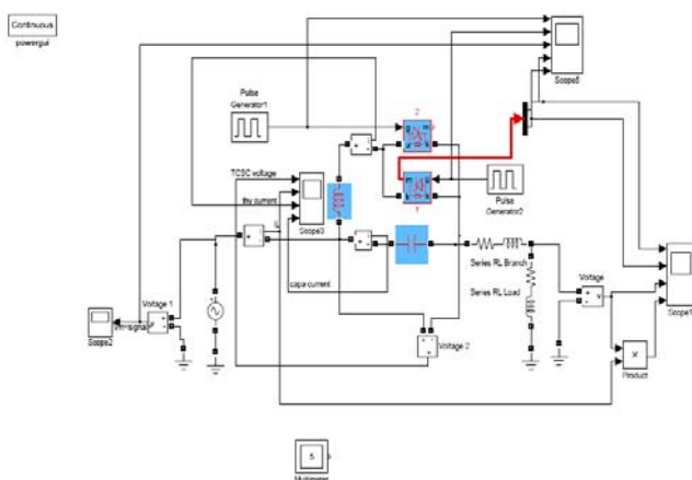
Fig. 5 Simulink model of TCSC device
