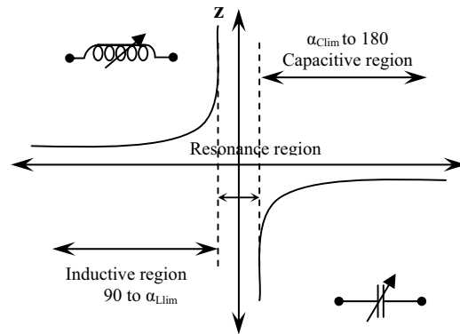
Fig. 4 Impedance Vs firing angle characteristic curve
