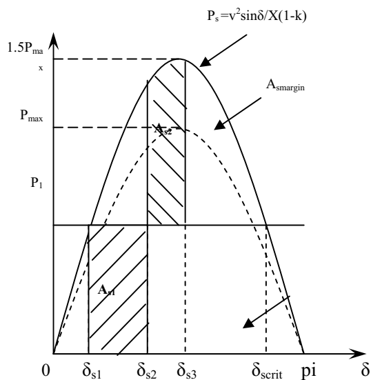
Fig. 9 Power Vs Angle curve with series compensation
