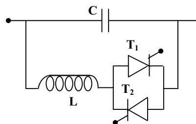
Fig. 1A simple diagram of TCSC device
