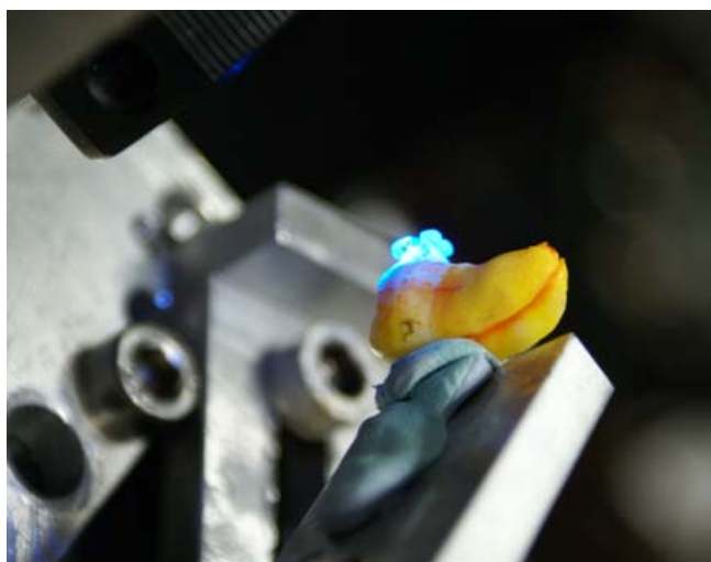
Fig. 2 OCT investigation of the samples using Fluorescence
