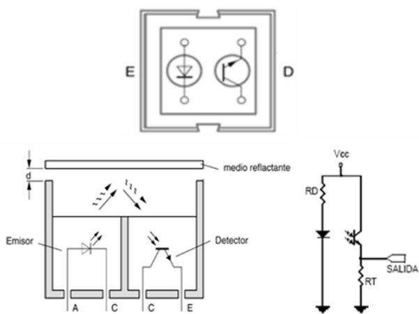
Fig. 1. Sensor CNY 70
