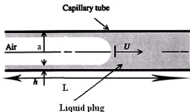
Fig. 5 Capillary model for a propagating liquid plug. Meniscus moves forward from left to right with a velocity of U , and leaves behind a film lining layer in the thickness of h . a , capillary tube radius; L , tube length
