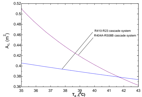
Fig. 3 Effect of condenser temperature (HTS) on condenser heat transfer area
