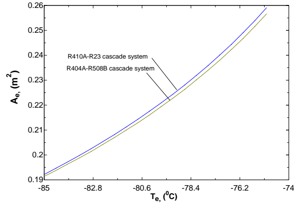
Fig. 8 Effect of evaporator temperature (LTS) on evaporator heat transfer area
