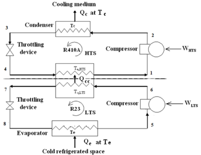
Fig. 1 Schematic diagram of cascade refrigeration system
