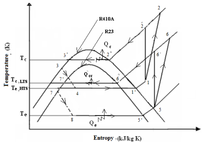
Fig. 2 Temperature-entropy diagram of cascade refrigeration system
