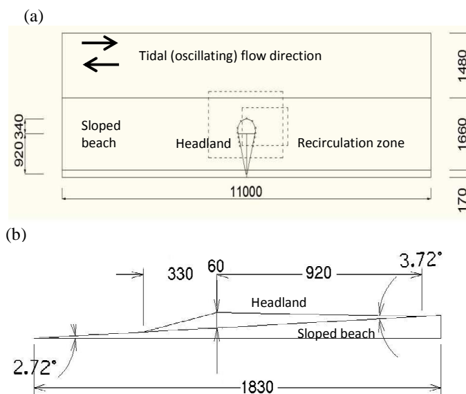
Fig. 1 Schematic diagram of the experimental set-up (a) flume and headland (b) side view of headland model and sloped beach. All dimensions in mm. Rectangles (with broken lines) over headland indicate field of view for experiments with high spatial variability (large rectangle) and low spatial variability (small rectangle) relative to flume and headland model
