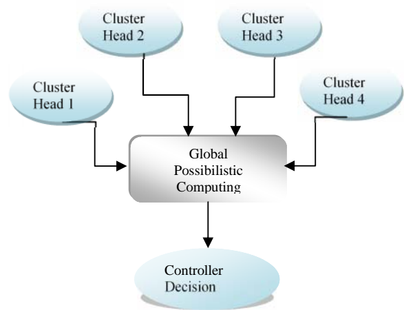
Fig. 5 Inter-clusters fusion
