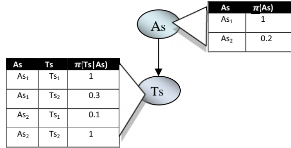
Fig. 1 A Simple possibilistic network
