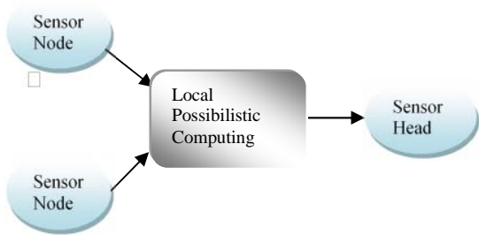
Fig.3 Intra-cluster fusion
