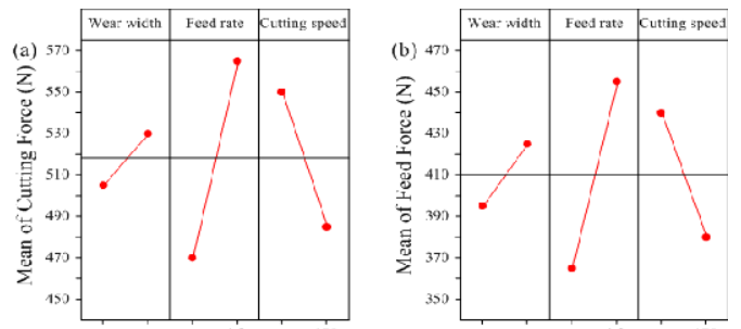
Fig.7 Main effect plots for force components (a) cutting forces (b) feed forces
