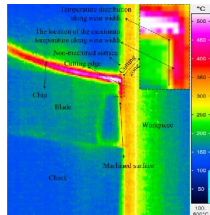
Fig. 4 Temperature measurement along wear width
