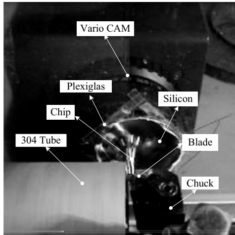
Fig. 2 Designed experiment to measure machining temperature
