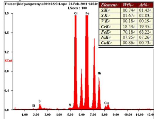
Fig. 3 The composition of austenitic 304 stainless steel
