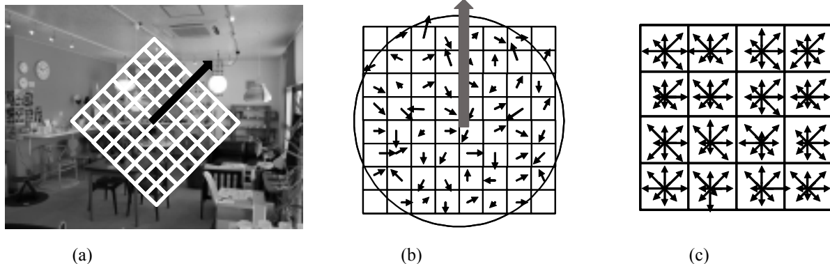
Fig. 1 Description of SIFT feature
