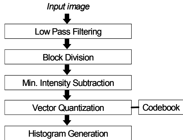
Fig. 2 Process steps of VQ histogram method
