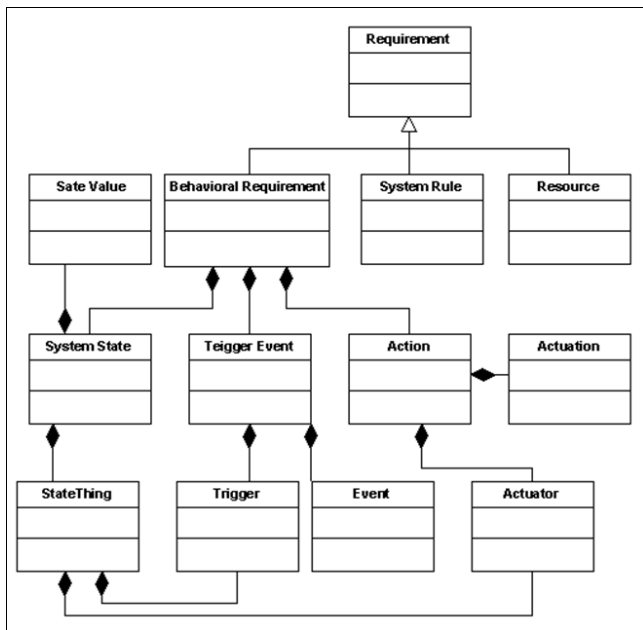
Fig. 2 Modeling Behavioral Requirements with UML
