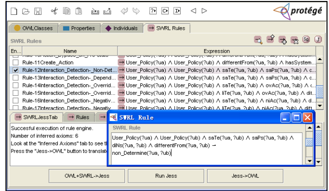
Fig. 3 Snapshot of Protégé and SWRLTab
