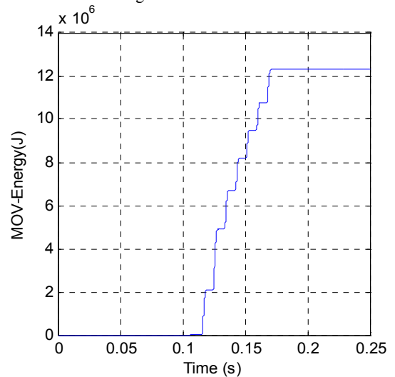
Fig. 11 Energy dissipated in the MOV
