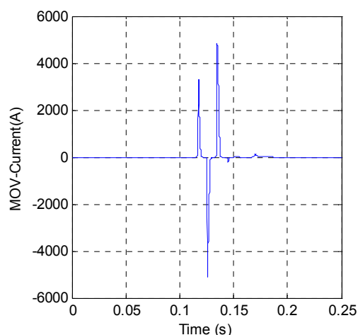
Fig 4 MOV-current
