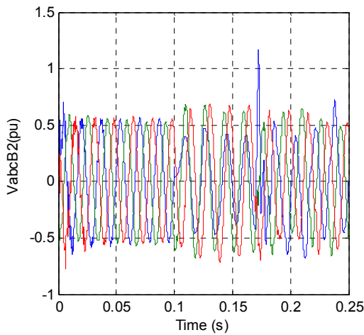
Fig. 7 Voltage at BUS2(pu)
