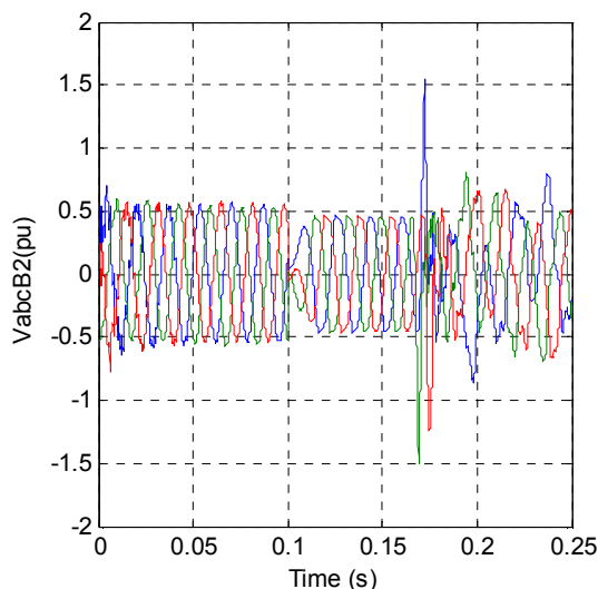
Fig. 13 Voltage at BUS2(pu)
