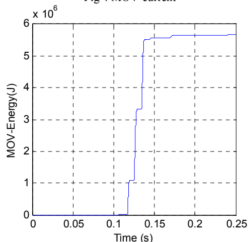
Fig. 5 Energy dissipated in the MOV
