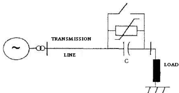
Fig. 2 Power system
