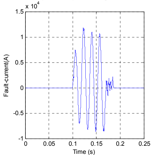
Fig. 14 Fault current
