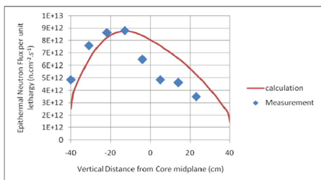
Fig. 7 Calculated and Measured axial epithermal neutron flux distributions for irradiation channel G3 – South side.
