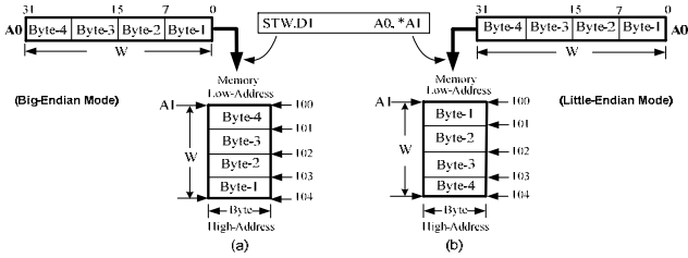
Fig. 7 Storing a word (W) of data in the memory in big and little endian mode
