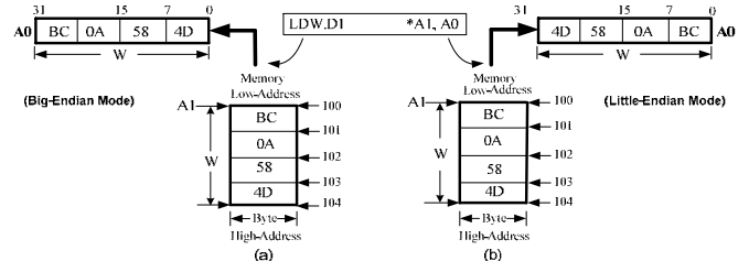
Fig. 13 Example of reading a word (W) from memory in big and little endian mode
