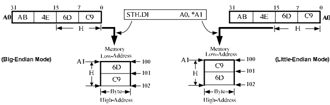
Fig. 11 Example of storing a half-word (H) in the memory in big and little endian mode
