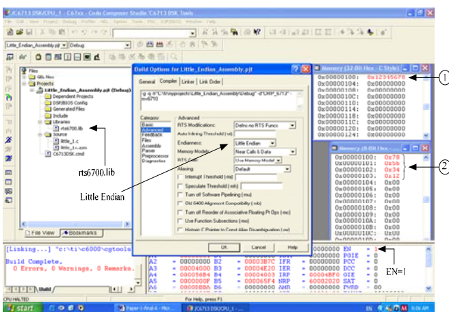
Fig. 4 A screen-shot of the CCS for little endian mode
