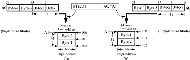
Fig. 8 Storing a half-word (H) of data in the memory in big and little endian mode
