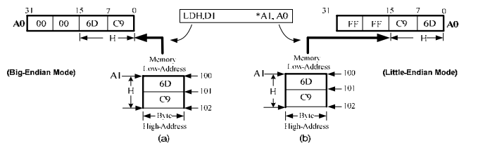
Fig. 14 Example of reading half-word (W) from memory in big and little endian mode
