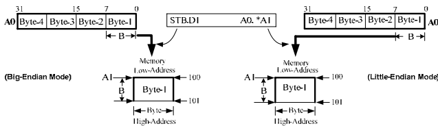
Fig. 9 Storing a byte (B) of data in the memory in big and little endian mode
