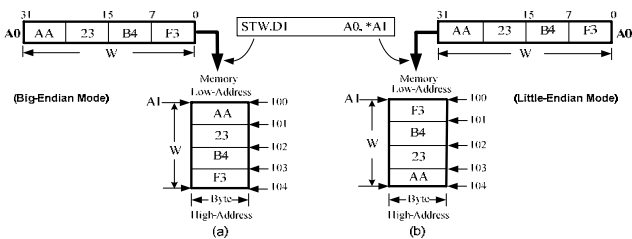
Fig. 10 Example of storing a word (W) in the memory in big and little endian mode
