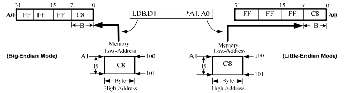
Fig. 15 Example of reading a byte (B) from memory in big and little endian mode
