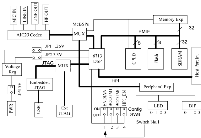
Fig. 1 Block diagram of the TMS320C6713 DSK board [12]
