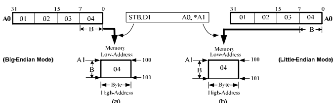
Fig. 12 Storing a byte (B) in memory in big/little endian mode
