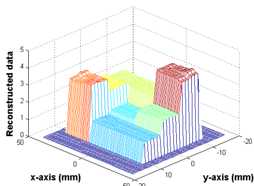
Fig. 3 Reconstructed relative permittivity distribution
