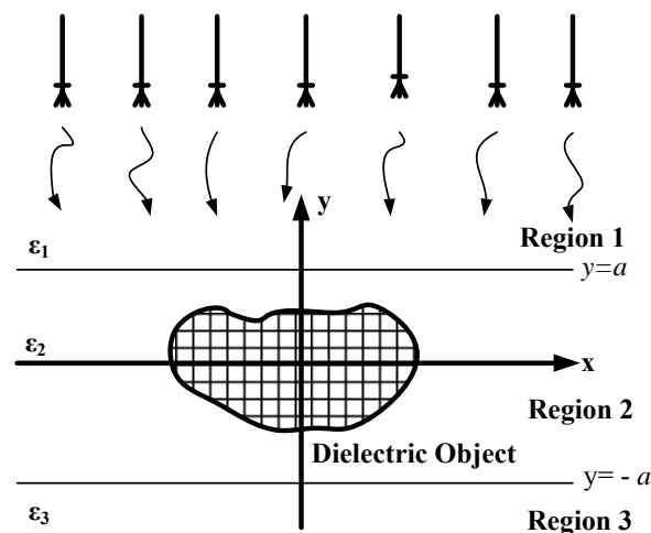
Fig. 1 Geometry of problem in the (x,y) plane
