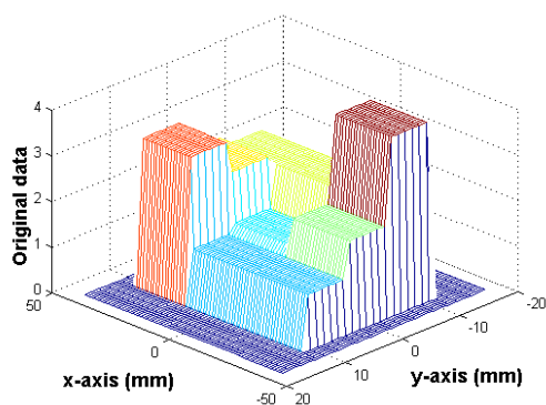
Fig. 2 Original relative permittivity distribution
