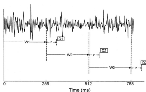
Fig. 1 Adjacent windowing technique [4]
