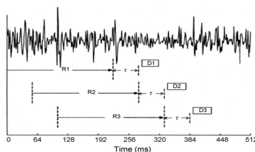
Fig. 2 Overlapped windowing technique [4]
