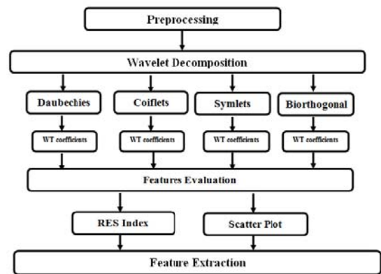
Fig.4 The procedures of SEMG feature extraction from wavelet coefficients using different MW
