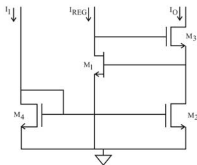
Fig. 1 Regulated cascode CM
