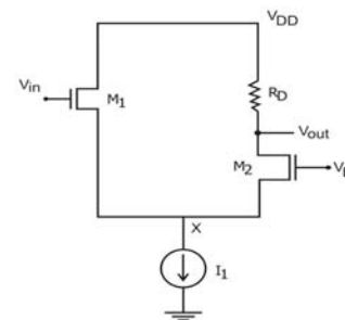
Fig. 2 Folded cascode
