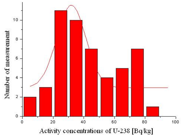
Fig. 4 Distribution of activity concentrations of ^{238}\text{U}
