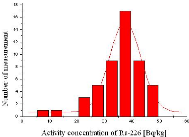
Fig. 3 Distribution of activity concentrations of ^{226}\text{Ra}
