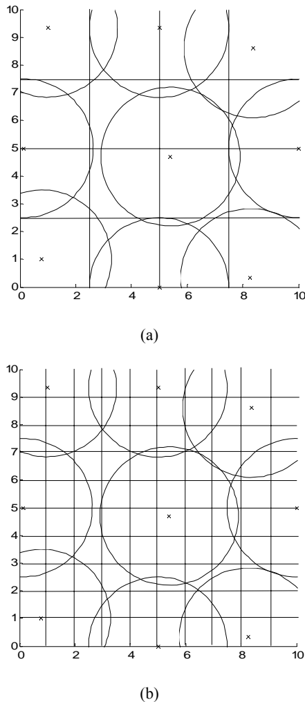
Fig. 1 Grid based coverage estimation for 9 sensors with sensing range equal to 2.5 in ROI of 10 \times 10 . (a) Grid size: 2.5 \times 2.5 ; coverage estimated: 100% (b) Grid size: 1 \times 1 ; coverage estimated: 95%
