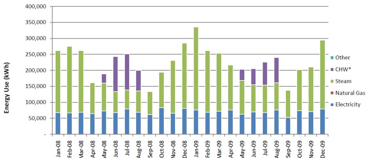
Fig. 3 Historical CMLP energy use (UWO, 2010).
