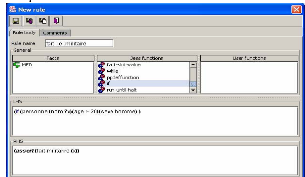
Fig. 5 screen of seizure of a rule
