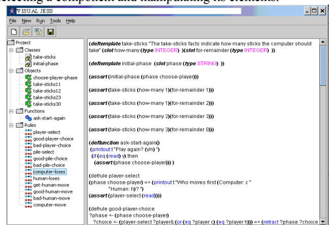
Fig. 1 main window of the application
