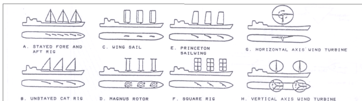
Fig. 1 Various sail rigs [19]
