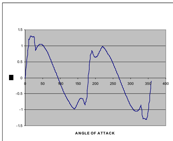
Fig. 3 Graph of the coefficients of lift (NACA 0018) with respect to angle of attack. (Reynolds number =6160000)
