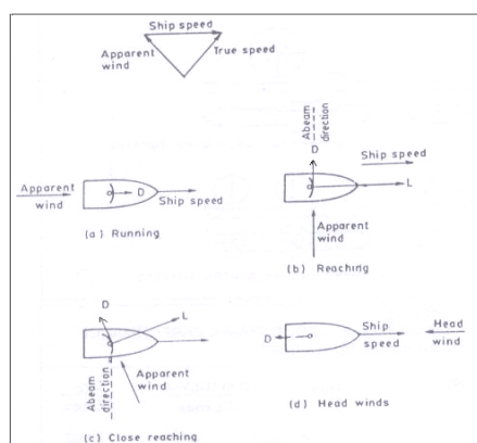
Fig. 2 Different modes of sailing (L and D denote lift and drag forces)
