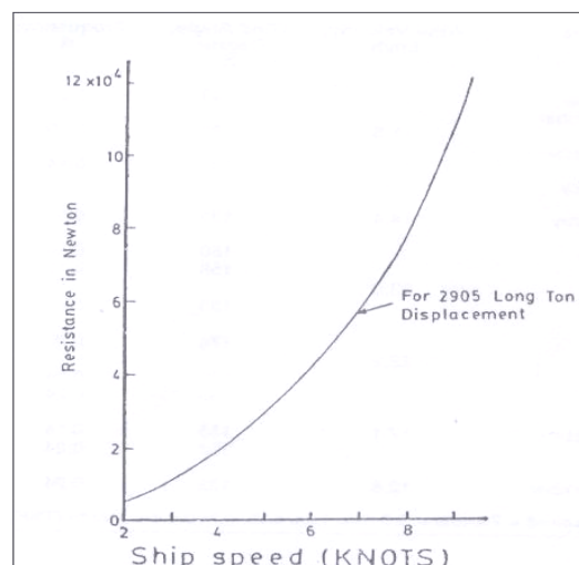
Fig. 6 resistance curve for minilace for 2951.48 t, 1 long ton = 1.016 ton
