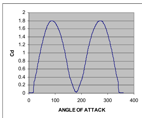
Fig. 4 Graph of the coefficients of drag (NACA 0018) with respect to angle of attack. (Reynolds Number =6160000)
