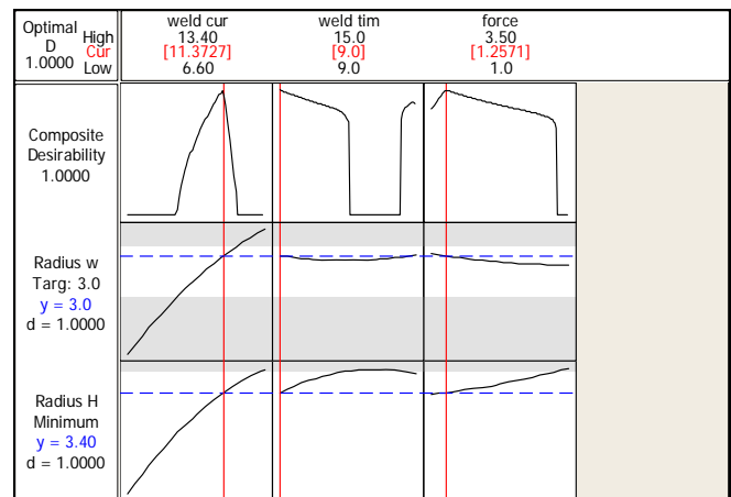
Fig. 6 Response optimization plot
