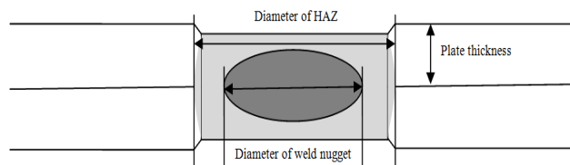
Fig. 1 Schematic illustration of the weld zone
