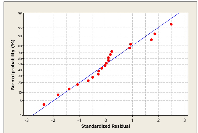
Fig. 5 Normal probability plot of standardized residuals for radius of HAZ
