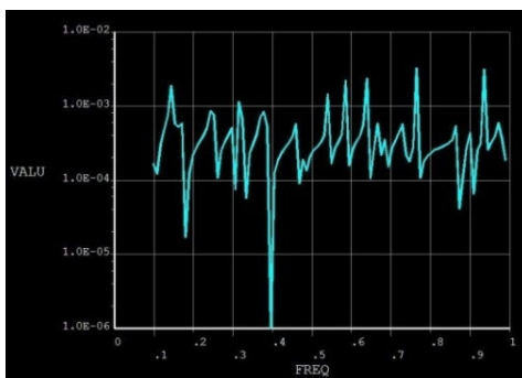
Fig. 15 Frequency Response (Log Scale)
