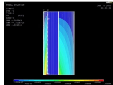
Fig. 24 Deformed Shape
