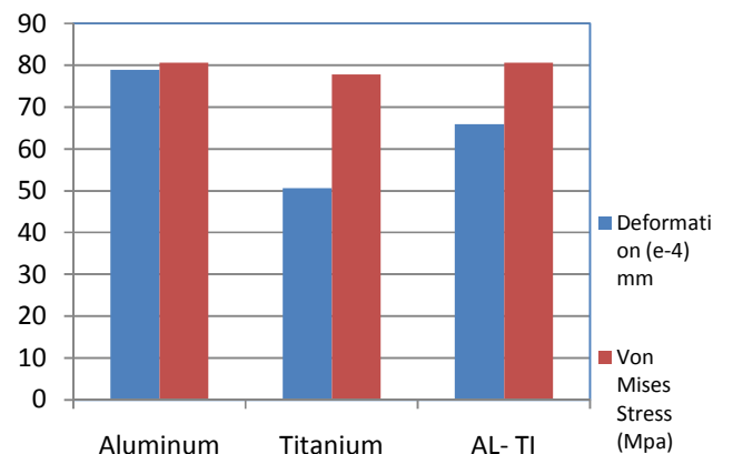
Fig. 12 Maximum von Mises Stress and Deformation Comparison Modal Analysis
