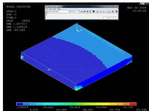
Fig. 6 Von Mises Stress Distribution of Aluminum Model
