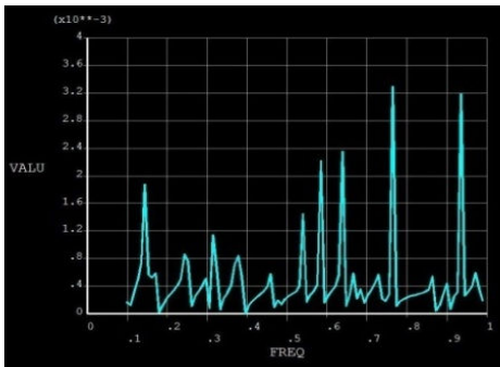
Fig. 14 Frequency Response (Linear Scale)
