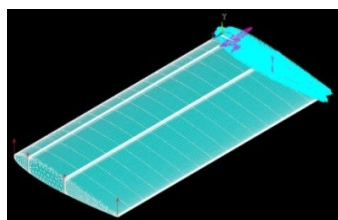
Fig. 5 Boundary Conditions
