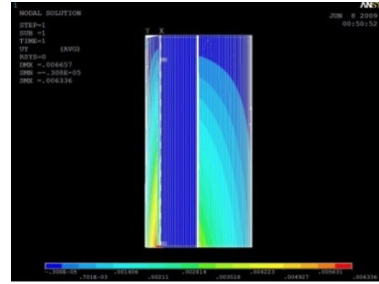
Fig. 22 Deformed Shape
