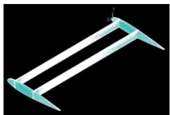
Fig. 4 Meshed Stiffeners and Spurs
