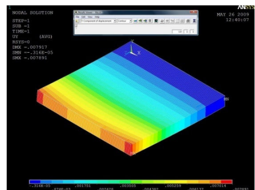
Fig. 7 Deformed Shape of Aluminum Model
