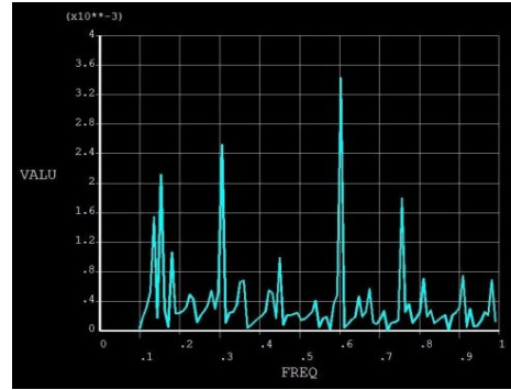
Fig. 16 Frequency Response (Linear Scale)
