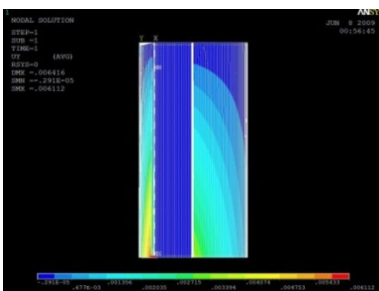
Fig. 28 Deformed Shape
