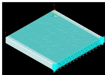
Fig. 1 Cantilever Plate
