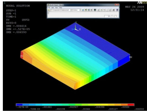
Fig. 11 Deformed Shape of Aluminum- Titanium (FGM)
