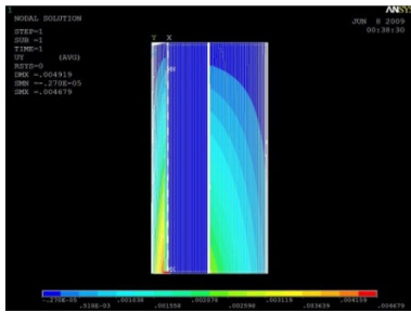
Fig. 26 Deformed Shape
