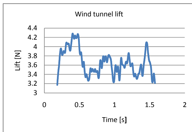
Fig. 19 Lift variation for the wind tunnel conditions
