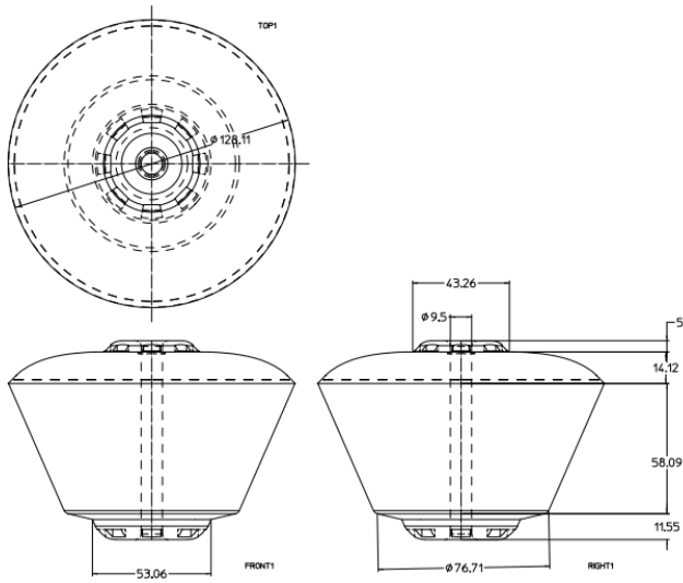
Fig. 2 Feeder geometry
