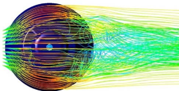
Fig. 5 Streamlines
