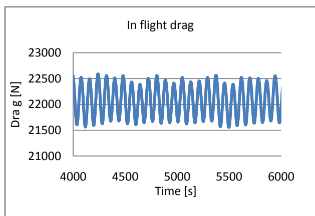
Fig. 9 Drag variation along time at 15 km altitude at constant speed of 10 m/s
