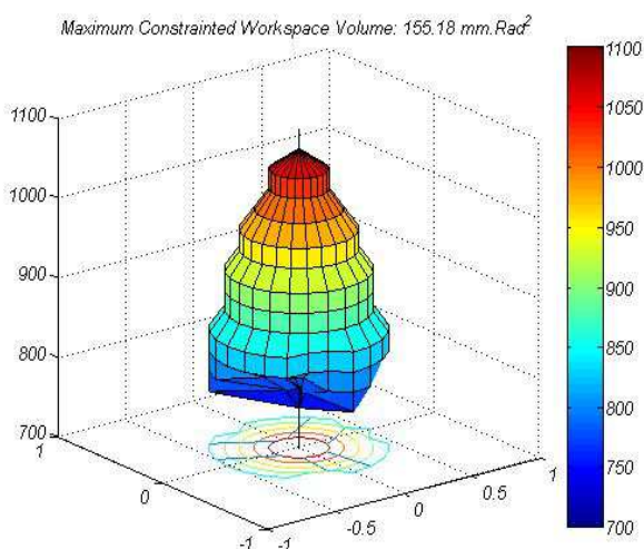
Fig. 9 Optimal workspace for the case study mechanism
