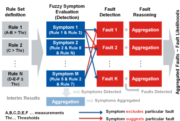
Fig. 7 AFDD engine – example
