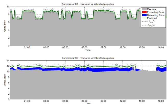
Fig. 6 Compressor amps draw monitoring
