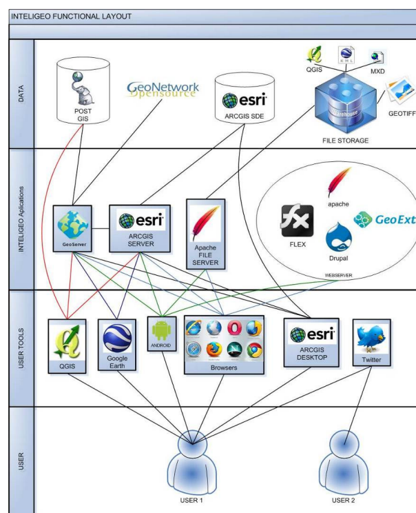
Fig. 6 Inteligeio functional Layout, which aggregates the best softwares from free and proprietary solutions [6]
