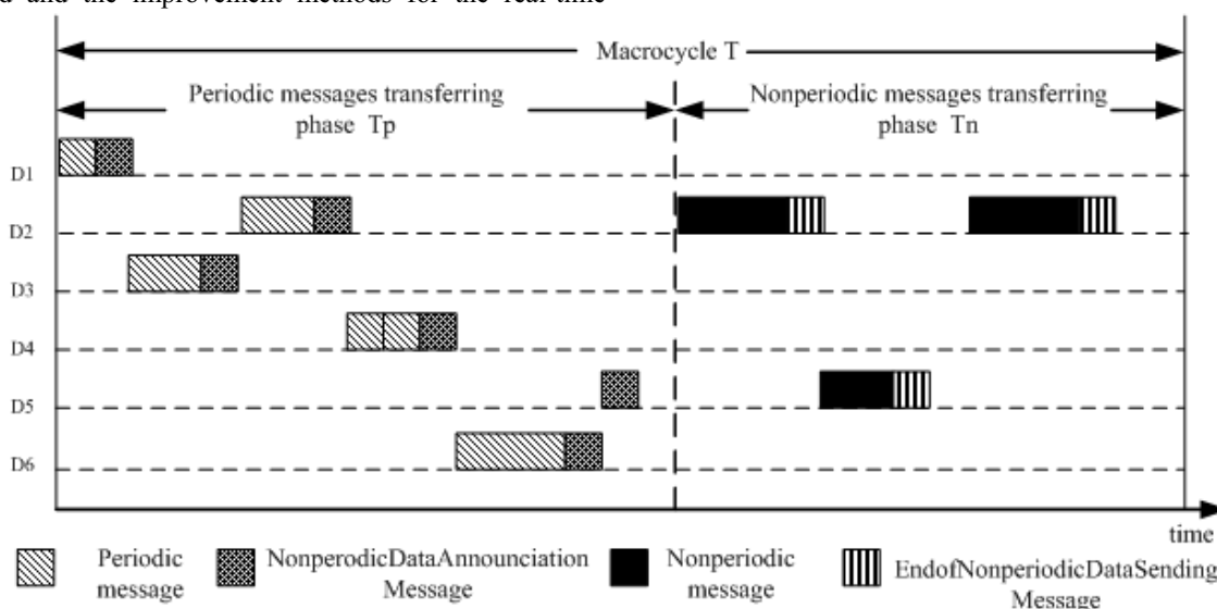
Fig. 1 EPA Deterministic Scheduling
