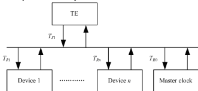
Fig. 3 Test of Time Synchronization Accuracy
