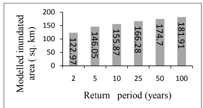
Fig.15 Modelled inundated area with respect to different return periods
