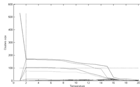
Fig. 3 The super-paramagnetic phase
