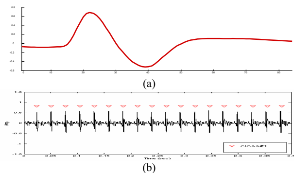
Fig. 4 Time localization of the spikes for example (1): (a) plot of the spikes, (b) time localization
