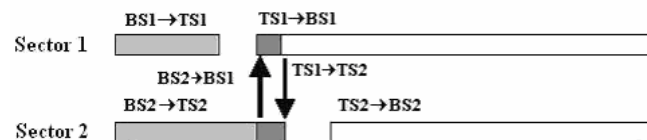
Fig. 3 Additional interference in ATDD [3]
