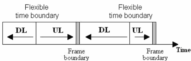
Fig. 1 Varying time boundary in ATDD frames [3]
