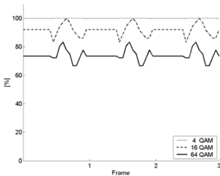
Fig. 7 Percentage of the covered area by different modulation in a three frame length time interval in case 'A'
