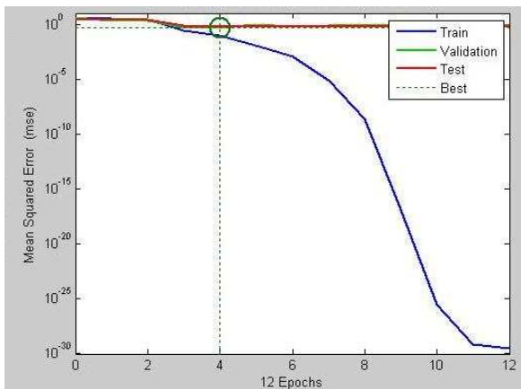
Fig. 5 Relationship between iteration and MSE
