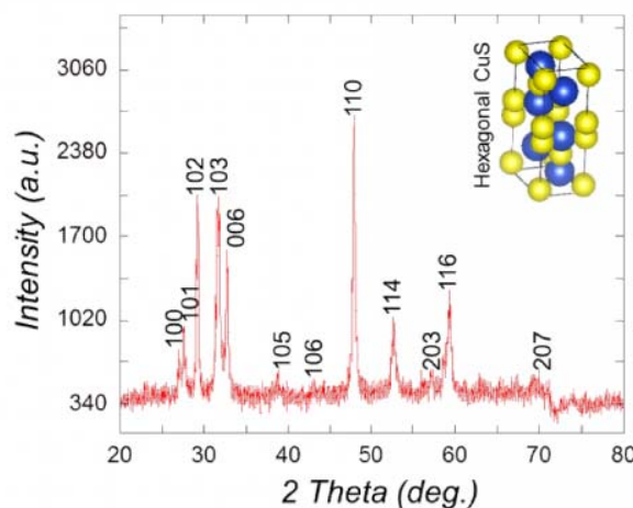
Fig. 3 XRD pattern for CuS nanoparticles, inset is a model of hexagonal CuS nanoparticles
