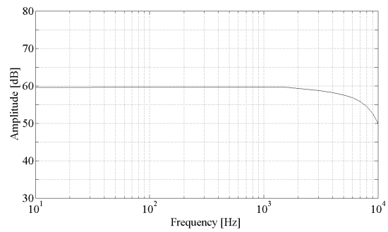
Fig. 4 Gain of the preamplifier and amplifier
