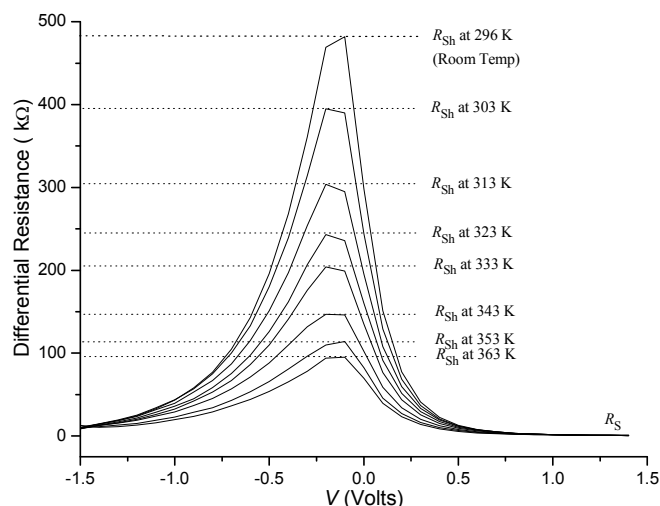
Fig.4 Dependence of differential resistance on voltage and temperature
