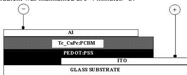
Fig. 2 Schematic diagram of fabricated Tc-CuPc:PCBM BHJ
