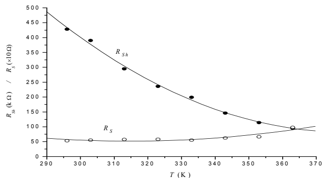
Fig. 9 Temperature dependence of BHJ resistances
