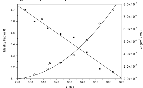
Fig. 10 Temperature dependence of ideality factor and mobility of BHJ
