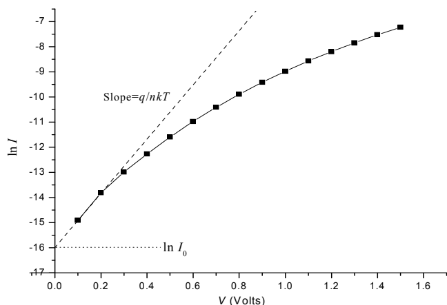
Fig. 5 Semi-log of room temperature dark I - V curves.
