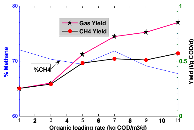
Fig. 10 Gas production and methane content
