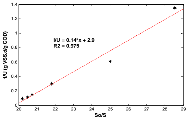
Fig. 5 Chen and Hashimoto model
