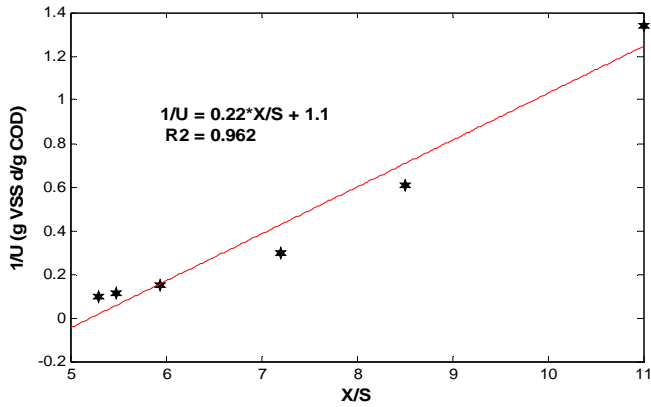
Fig. 4 Contois model
