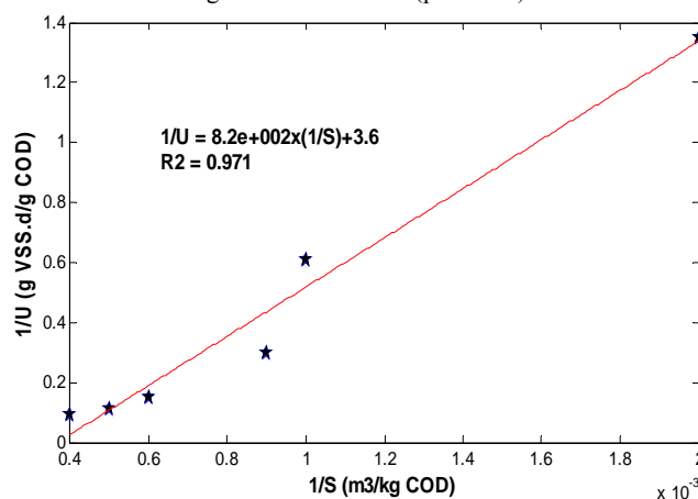
Fig. 3 Monod model
