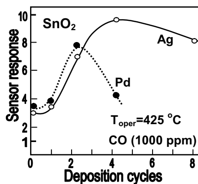
Fig. 3 Influence of SnO 2 surface modification on sensor response to CO
