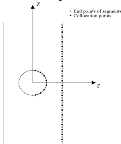
Fig. 2 Discretized representation of the vapour bubble and internal surface of the vertical rigid cylinder in the cases
