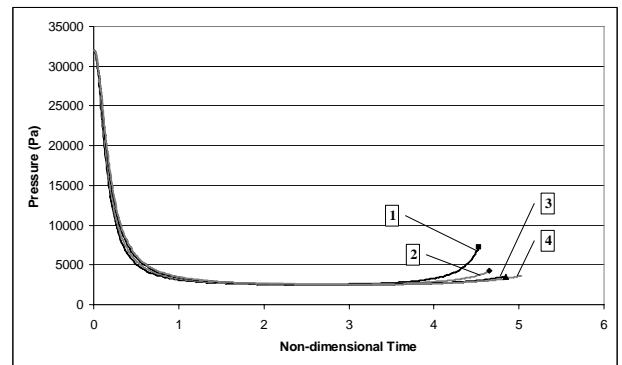
Fig. 8 Variation of internal pressure of a single cavitation bubble inside a vertical rigid cylinder against non-dimensional time in the absence of buoyancy forces in the cases of (1) \lambda = 3 , (2) \lambda = 2.5 , (3) \lambda = 2 , (4) \lambda = 1.75
