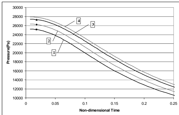
Fig. 10b Variation of pressure at the intersection point of radial axis and internal surface of the vertical rigid cylinder against non-
