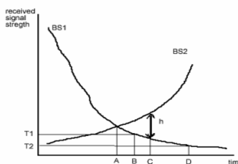
Fig.1 Movement of a MS in the handoff zone
