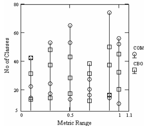
Fig. 4(b) COM and CBO Metric Ranges
