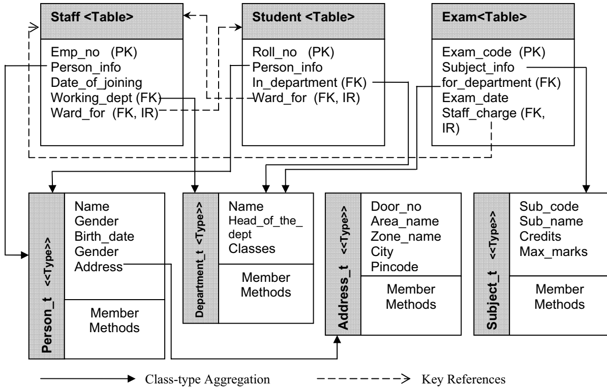
Fig. 2 Sample Schema for the Metrics Evaluation
