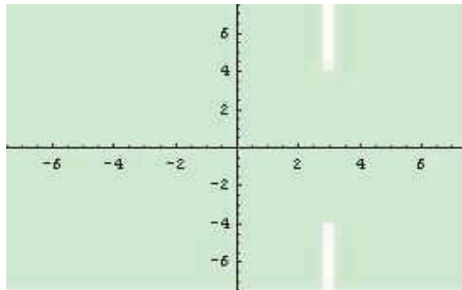
Fig. 2 ( \alpha = -2 )
