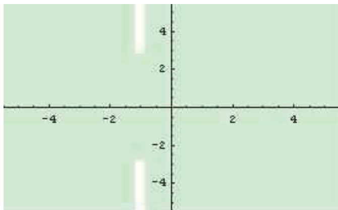
Fig. 1 ( \alpha = 2 )
