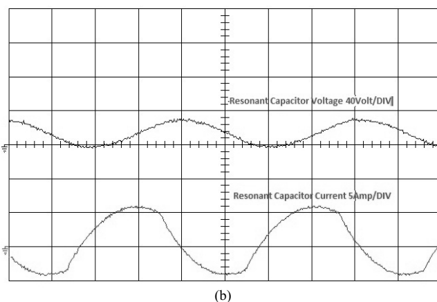
Fig. 3 (a) Simulation results of Resonant Capacitor Current and Voltage (b) Experimental results of Resonant Capacitor Current and Voltage, 2\mu s (time/DIV)
