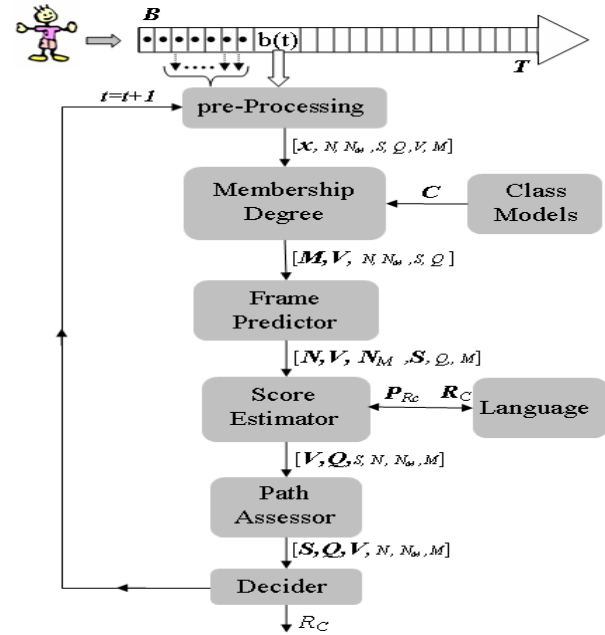
Fig. 1 Components and flow diagram of a recognition machine (C=Class Models; b , X =raw and processed current input frames; M =Membership degrees; V =Current Predicted Induces of Frames; N =Next Predicted Indexes; N_M =Membership Degree of Next Indexes; S =Scores; Q =Path Assessors; R_C =Recognized Class)
