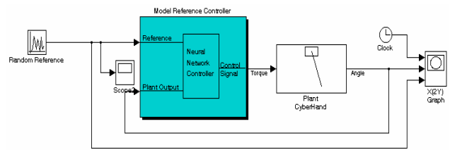
Fig. 11 Using neural network for cybernetic hand control
