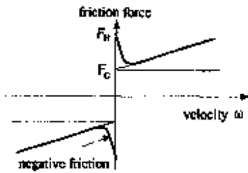
Fig. 2 Friction variation in different motion stage is a function of angular velocity [12]
