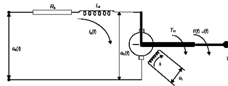
Fig. 5 Elbow joint drive motor illustration
