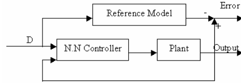
Fig. 10 A complete illustration of system and controller
