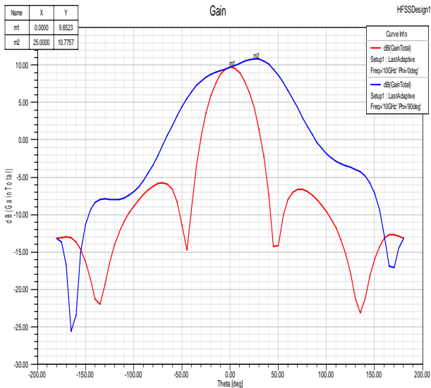
Fig. 6 (c) Gain of 1x2 Grooved patch Array
