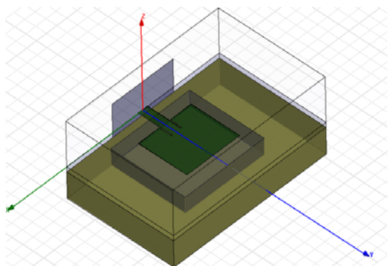
Fig. 3(a) Grooved Microstrip patch antenna with CPW inset feed
